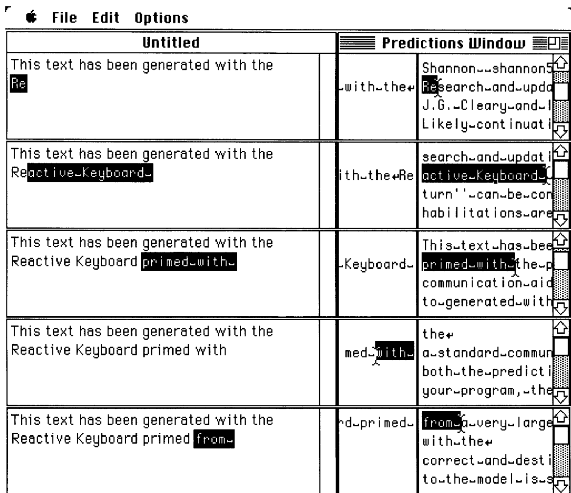
Figure 10. Using RK-POINTER, the Macintosh version of the REACTIVE KEYBOARD
