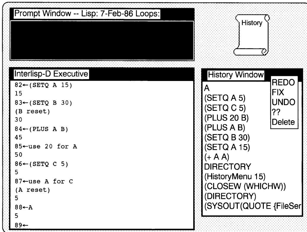
Figure 2. A portion of the INTERLISP-D environment, showing HISTMENU in use
