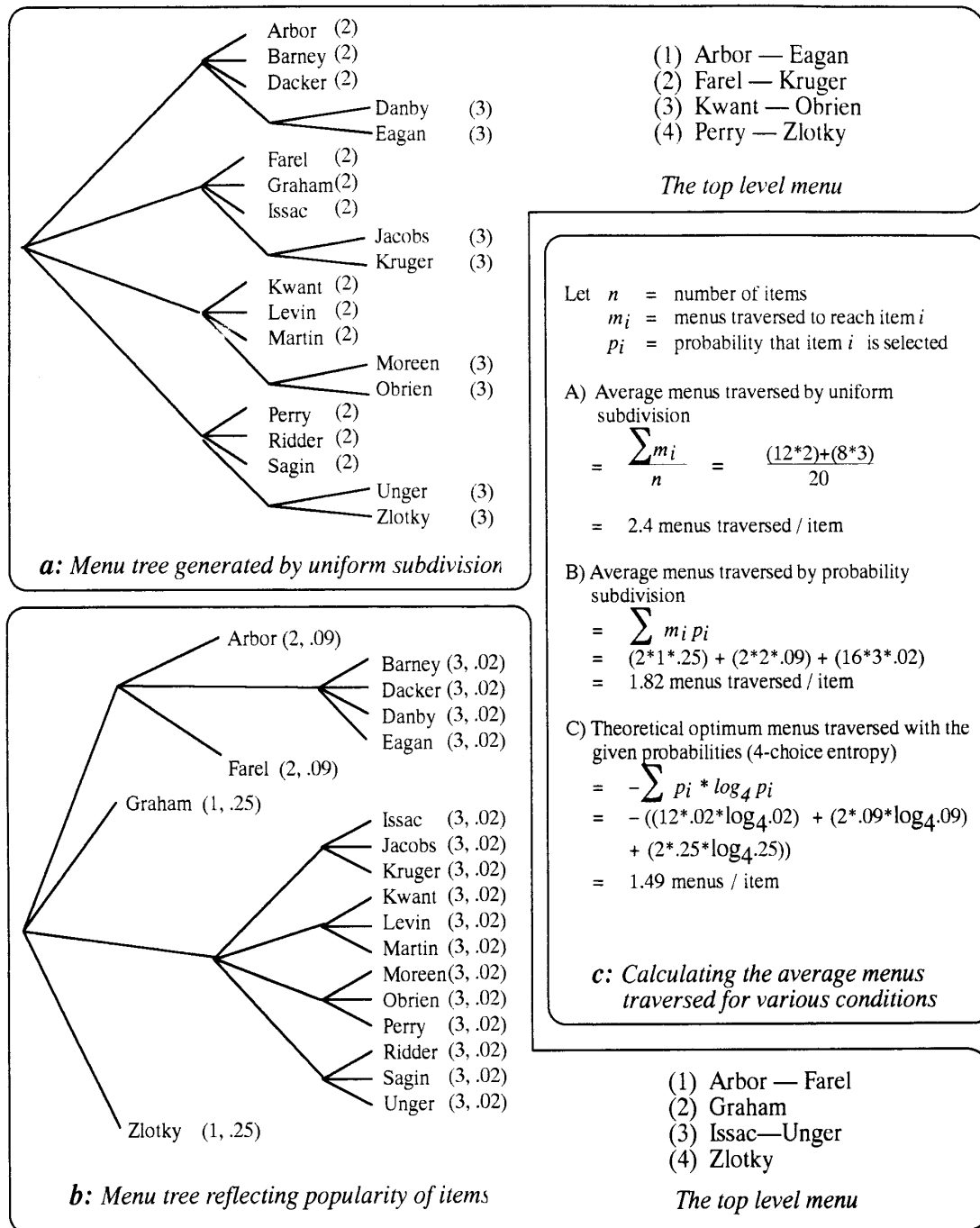
Figure 8: Menu trees generated by uniform and probability subdivision
