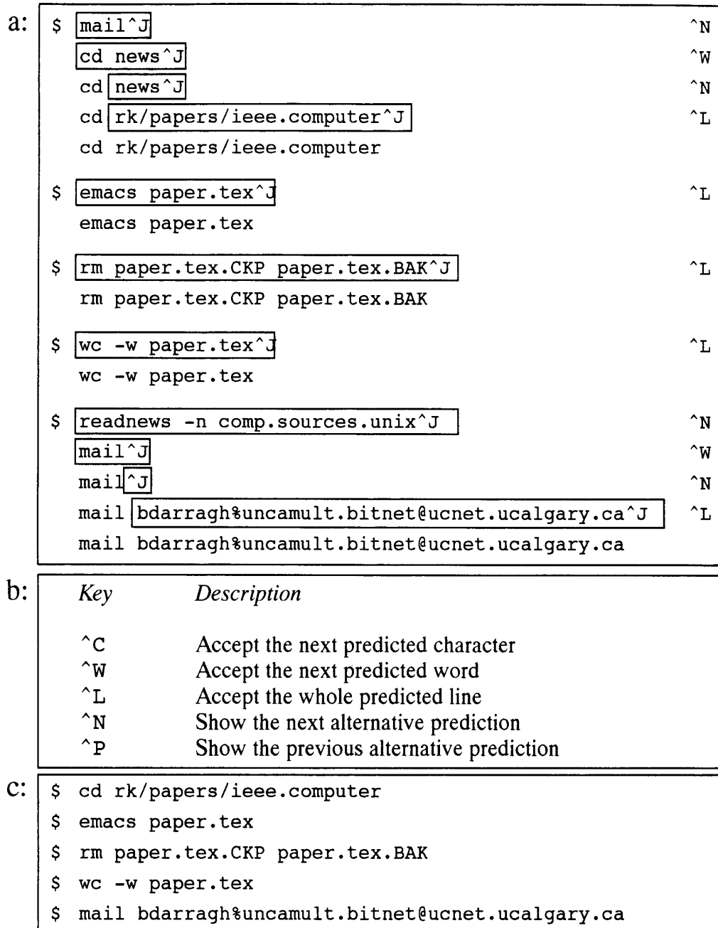
Figure 9. Using RK-BUTTON, the UNIX version of the REACTIVE KEYBOARD. a) an RK-BUTTON dialog with UNIX b) a key to several commands dealing with predictions c) screen contents at end of the dialog
