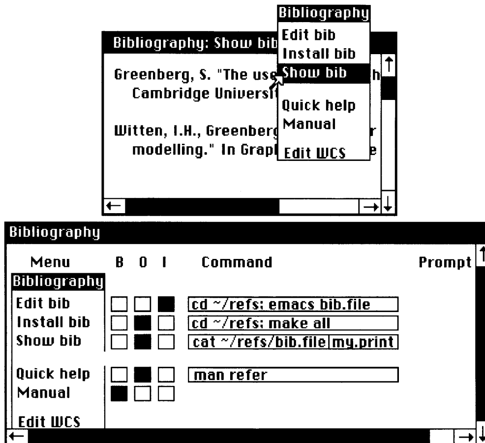
Figure 12: The Workbench Creation System. The top window show a workbench and menu for managing bibliographies, while the bottom one shows the editor associated with that workbench.
