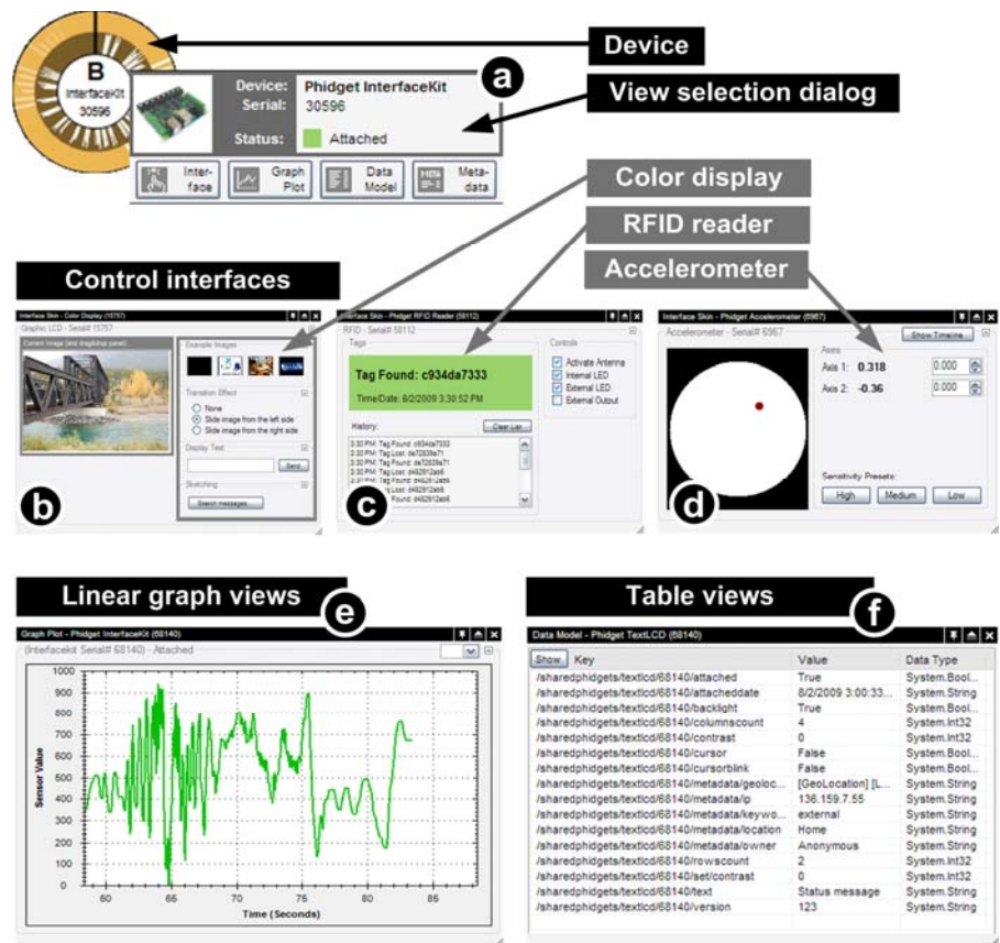
Figure 6. Details-on-demand.
