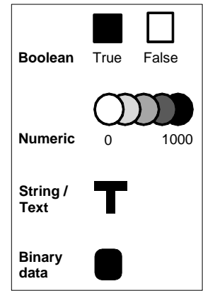
Figure 7. Event encoding.
