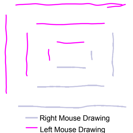
Figure 6. Diagonal Partitioning
