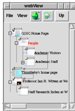
Figure 3: Cross-site link indicators
